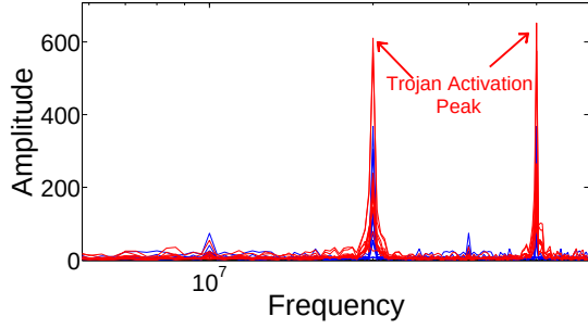
Figure 4: A2 Trojan detection in frequency domain.
