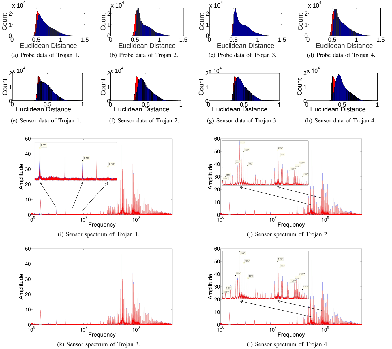
Figure 6: Trojan detection results with external probe (top row), on-chip sensor (middle row) and sensor spectrum (bottom row).
