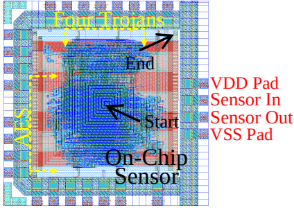
Figure 3: Layout of the circuits with on-chip sensor integrated.
