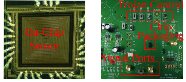
Figure 5: Die image of the fabricated AES (left) and the customized PCB with chip-on-board packaging (right).
